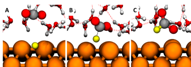
Figure 2. Snapshots of the reactive intermediates in the formate formation pathway from QM R \mu D simulations at 298 K and pH 7. The colors are Cu in orange, C in gray, O in red, and H in yellow (involved in reaction) or white (in water). Hydrogen bonds (HBs) are denoted as red dashed lines. (A) Initial state (CO 2 + H*). (B) Transition state (TS). (C) Final state (HCOO - ). \Delta G^\ddagger = 0.80 eV from (A) to (B). The C–H forming bond is 1.56 Å in (B) and 1.10 Å in (C). Notice that several HBs to solvent water play an important role in the energetics.
